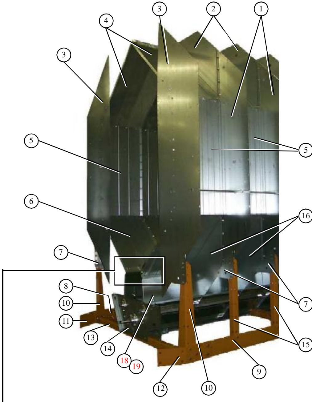
This photograph was taken before the front plenum end panel and outer screens were installed in order to get a good view of the inside screens and bulkheads.
